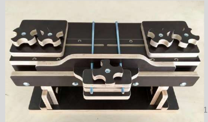
DEVICES FOR GROOVE CUTTING AND DOMINO TENSION INSERTION
