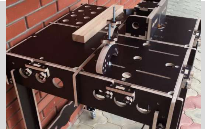
DEVICES FOR GROOVE CUTTING AND DOMINO TENSION INSERTION
